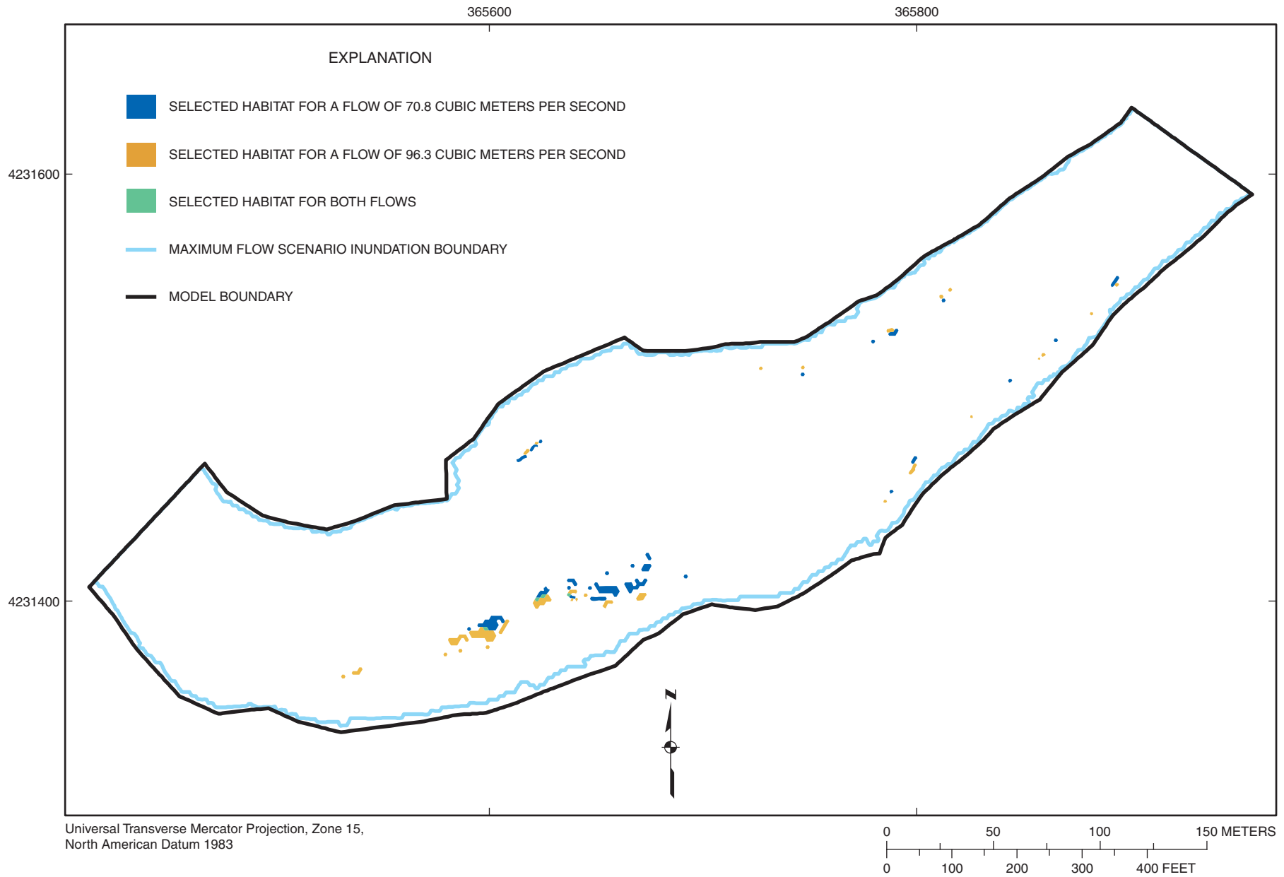
Figure 4-91. Selected habitat area distribution for habitat category 22 (channel catfish) at flows of 70.8 and 96.3 cubic meters per second at Marais des Cygnes River site MDC2.
